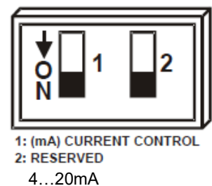
Fig. 7. Dip switches (view with PCB at bottom)
