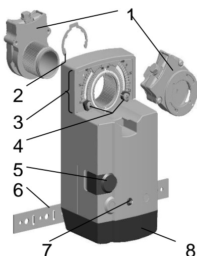
Fig. 2. Setting units and control elements
