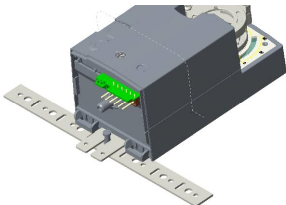
Fig. 12. Actuator with access cover removed
