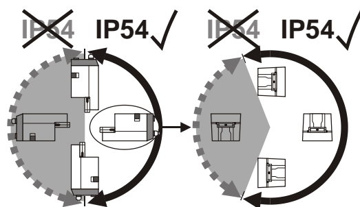
Fig. 10. Mounting for IP54
