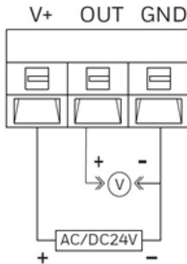
0-10V
