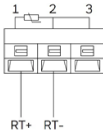
NTC10K/NTC20K/PT1000 Two-wire Circuit
