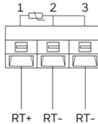
NTC10K/NTC20K/PT1000 Three-wire Circuit
