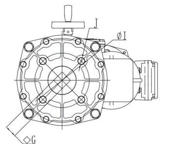
NOM16(25)H0200P/NOM16(25)H0400P/NOM16(25)H0600P/NOM16(25)H0800P/NOM16(25)H1000P
