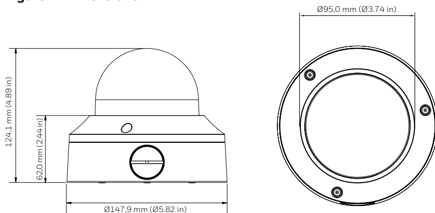
Figure 1. Dimensions
